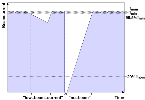
Figure 1: A “no-beam” failure starts when the beam current drops below 20% of the nominal beam current I_{\text{nom}} ; a “low-beam-current” already below 99.5% of the nominal lower current limit I_{\text{min}} (if it isn’t a “no-beam” failure). Both modes stops when the nominal beam current I_{\text{nom}} is reached again.
