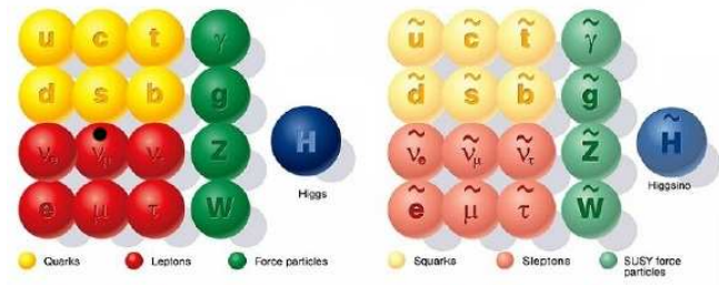
Standard particles SUSY particles
