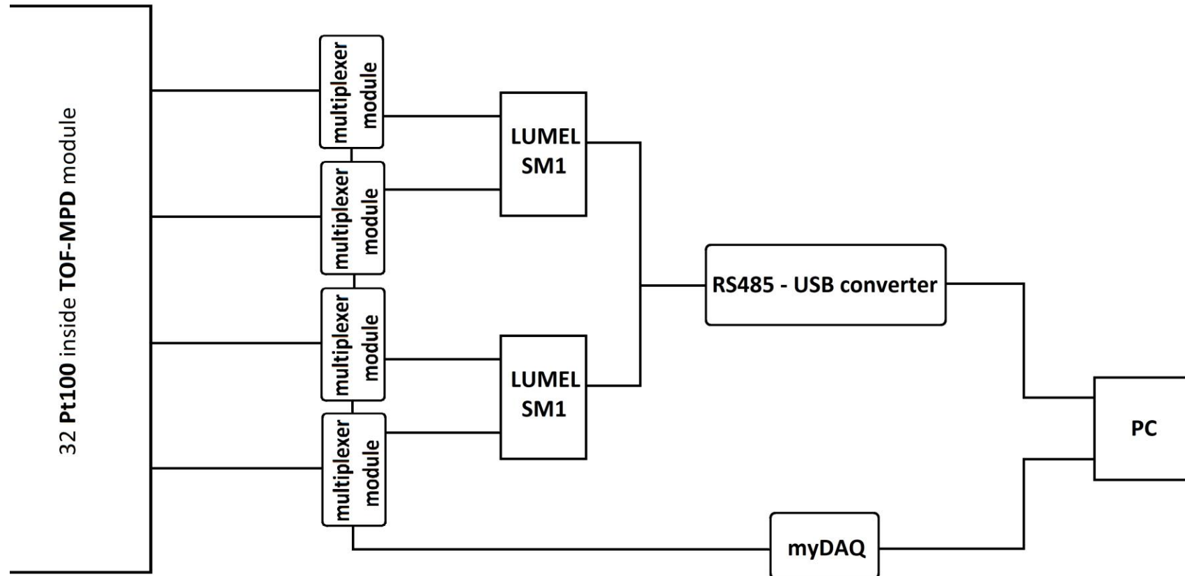
Figure: Electrical block diagram of the device
