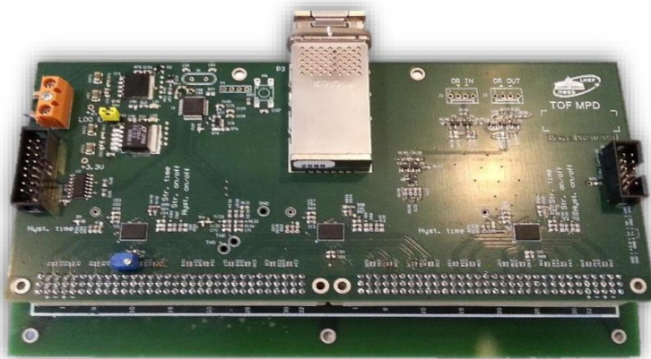
Preamplifier board (ref. TOF MPD Collaboration JINR)
