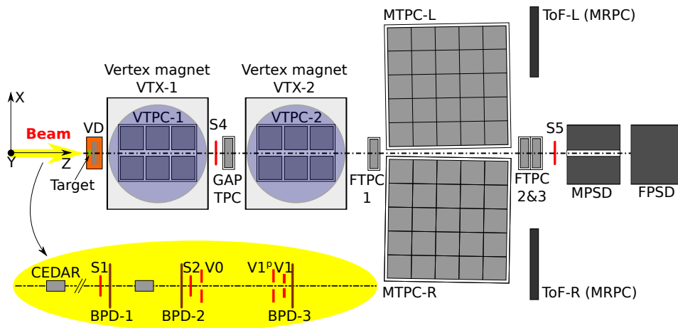
Fig. 1. NA61/SHINE detector subsystems after LS2 upgrade.
