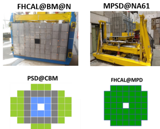
Fig. 1. Photo of assembled FHCAL for the BM@N experiment and MPSD for the NA61/SHINE experiment, upper figures. Schematic views of the PSD@CBM and FHCAL@MPD, down figures.
