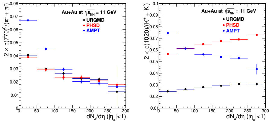
Fig. 1. \rho(770)/\pi (left) and \phi(1020)/K (right) ratios as a function of multiplicity in Au+Au collisions predicted by UrQMD, AMPT and PHSD event generators.
