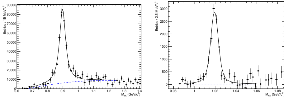
Fig. 2. Examples of invariant mass distributions for opposite-sign \pi K (left) and KK (right) pairs after subtraction of the mixed-event background in the p_T range 0.1-0.3 GeV/c. Peaks from decays of K^*(892)^0 and \phi(1020) mesons are fit to a combination of Voightian function and polynomial.
