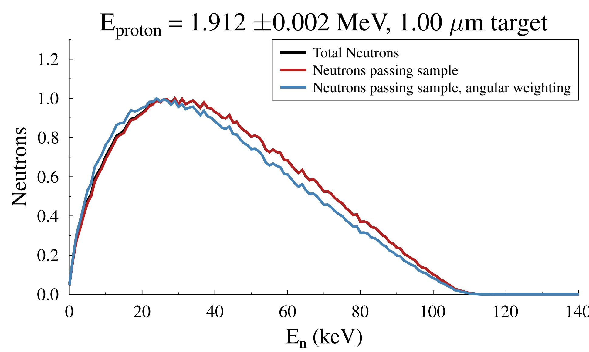
Figure 2: Comparison of the number of angle-integrated neutrons per linear energy bin for a simulation that contain weighting and no weighting for a sample with a radius of 3 mm. The radius of the Li-spot is 3 mm. The simulated spectrum is normalized to a common maximum of 1.
