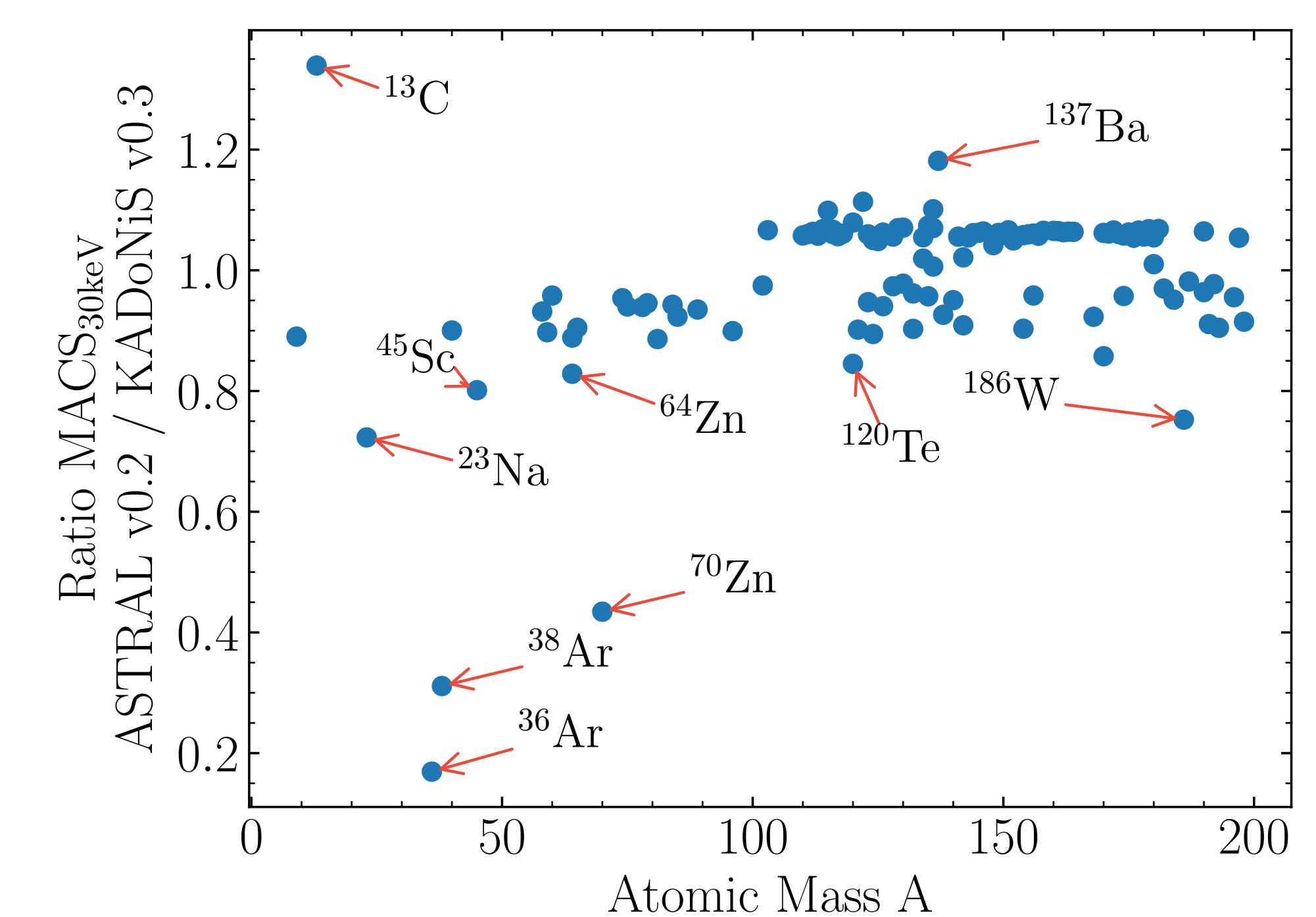
Figure 3: Comparison of MACS at kT=30 keV from the present ASTRAL v0.2 and the KADoNiS v0.3 compilation [3].
