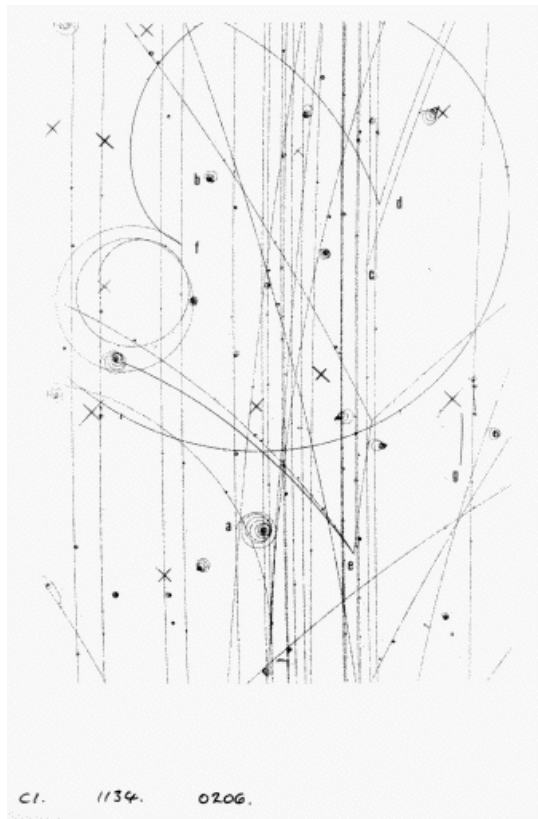
Bubble chamber photograph
