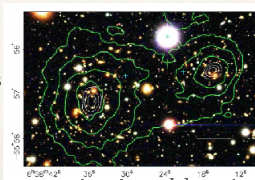
gravitational lensing
