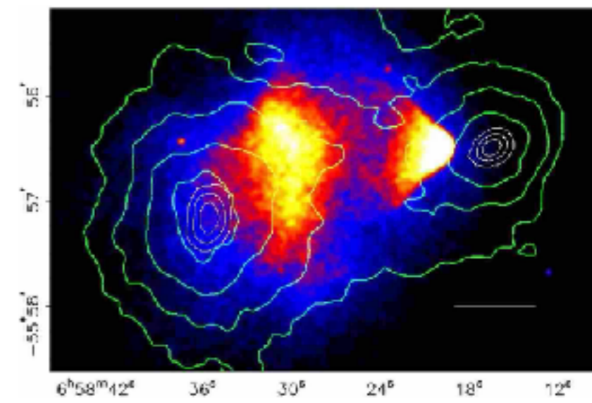
X-ray
