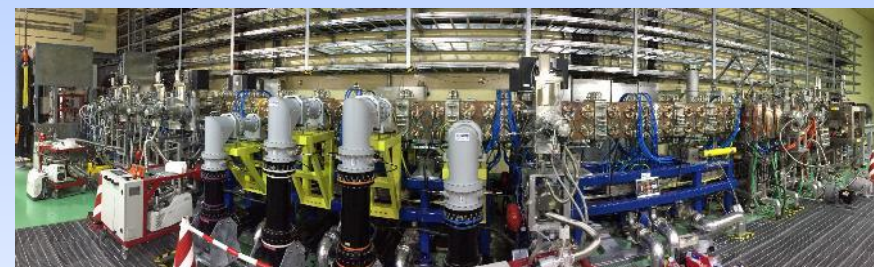
LIPAc accelerator
