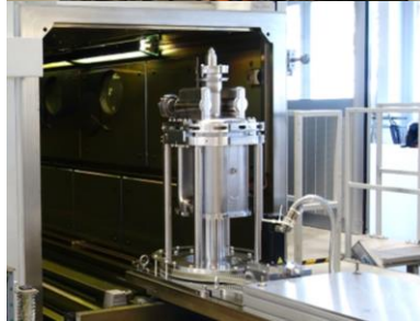
e-beam welding
