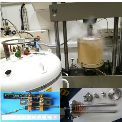
Mechanical testing
