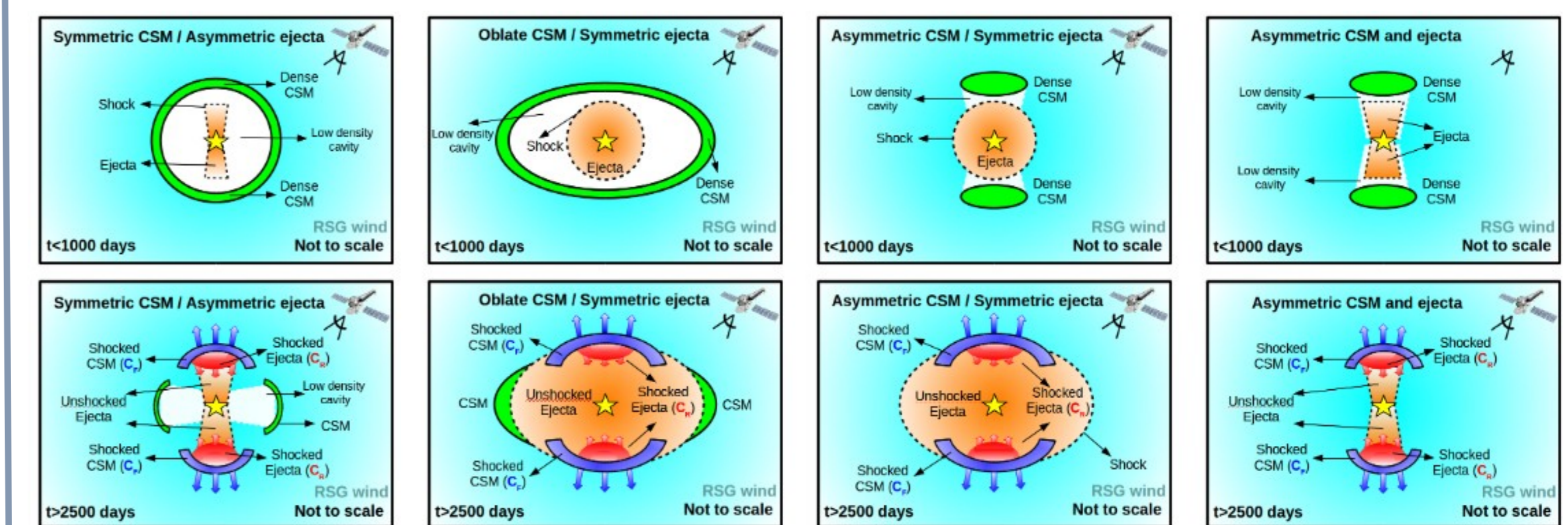
Figure 7: Cartoon depicting four possible geometrical scenarios to generate the X-ray emission of SN 1996cr. Top and bottom panels show the SN explosion before and after the interaction with the dense CSM, respectively.
