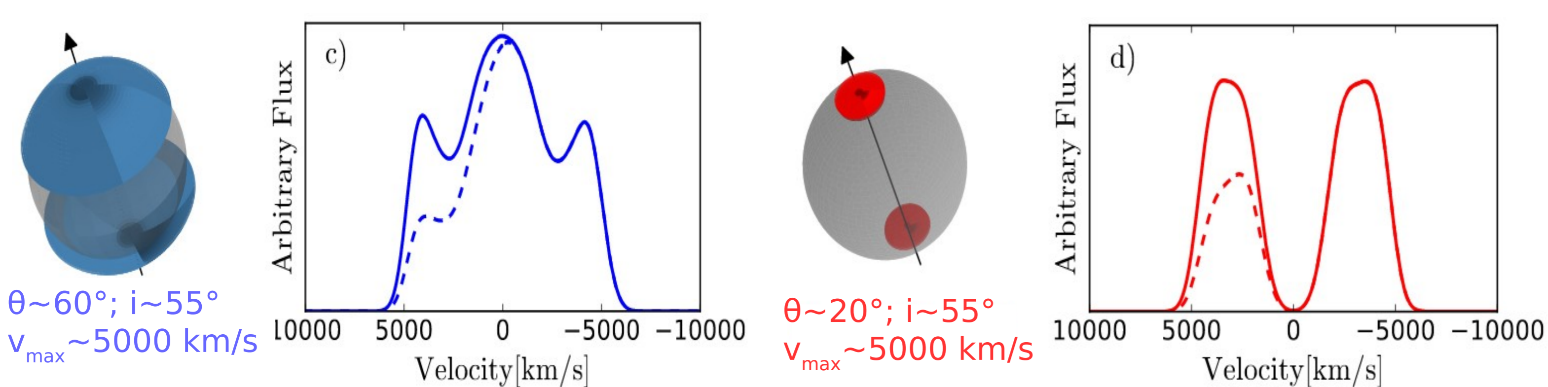
Figure 3: Examples of polar expanding shock structure geometries and their associated profiles (using shellblur model) which explain well the X-ray emission line profiles of SN 1996cr. Dashed lines indicate internal uniform density obscuration by N_{\text{ejecta}} = 1e23 \text{ cm}^{-2} .
