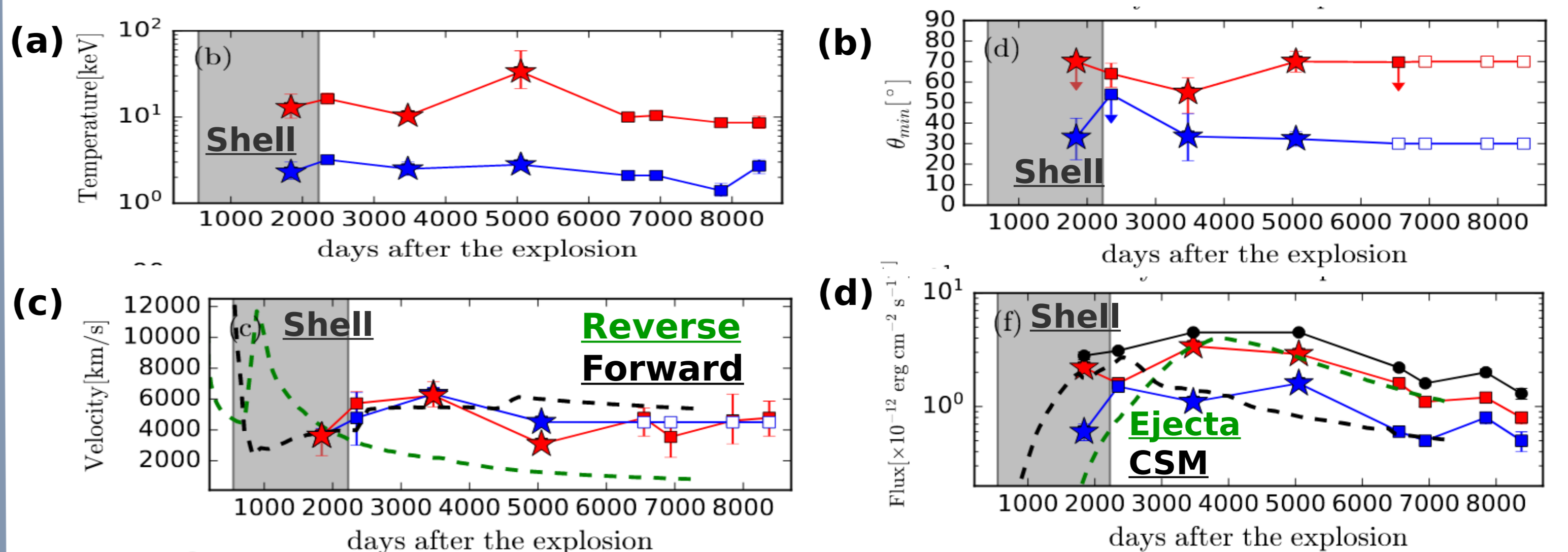
Figure 6: Evolution of temperature (a), \theta_{\min} (b), expansion velocity (c) and flux (d) for components C_R (red) and C_F (blue). Dashed black and green lines denote 1-D model predictions by Dwarkadas et al. 2010 (hereafter D10; MNRAS,407,812); in (c) they denote the forward and reverse shock velocities, respectively; in (d) they are the fluxes from the CSM and ejecta, respectively.
