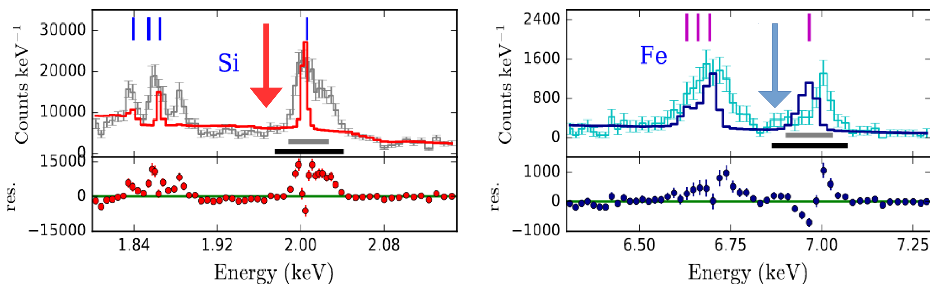
Figure 2: Close-up spectra of the H-like and He-like emission complexes for Si and Fe (grey and cyan spectra). Red and blue solid lines representing a simple NEI model (vpshock) at native HETG resolution. As highlighted by the arrows, the high velocity redshifted side of the profile is partially/completely obscured.
