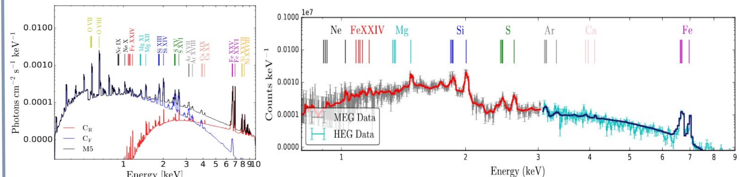
Figure 4: Left: Best-fit model M5 (black curve), with components C_R (red curve) and C_F (blue curve). Right: the best-fit model M5 compared to the 2009 epoch HETG spectra.
