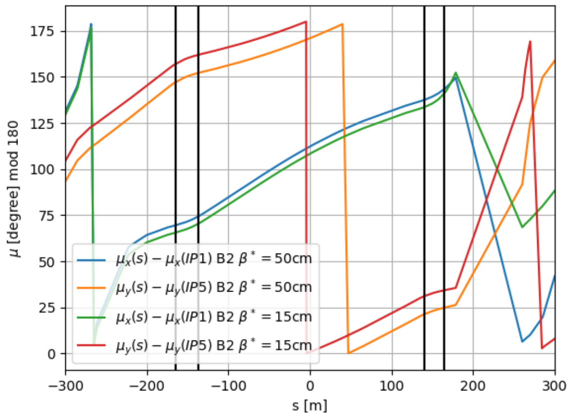
Phase advance from IP
