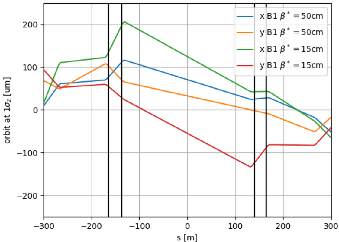
Single cavity orbit residual (right side) V=3.4 MV
