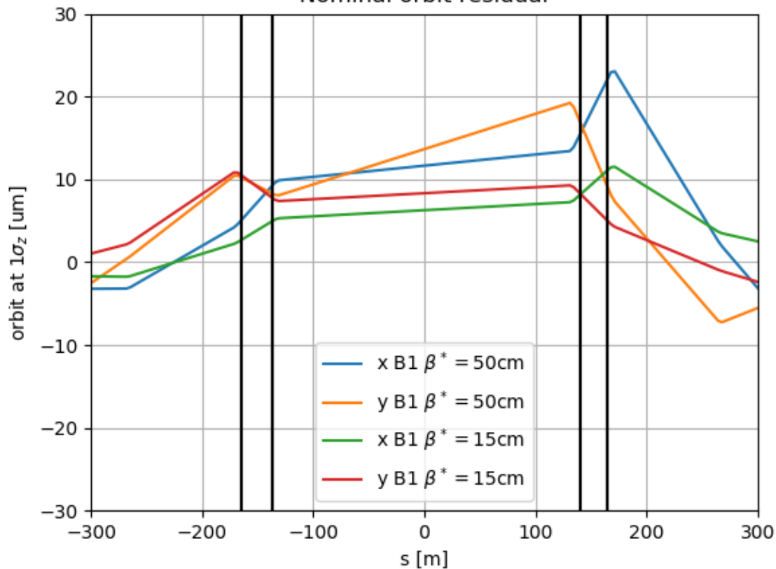
Nominal orbit residual
