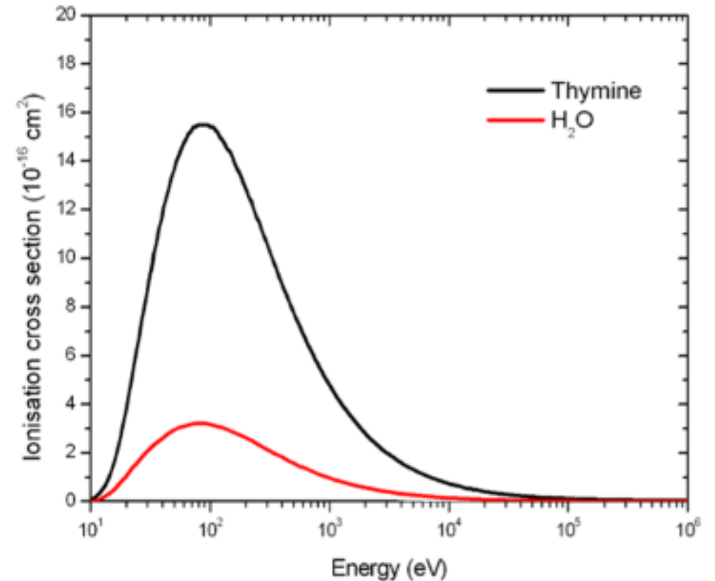
Electron ionisation total cross section
