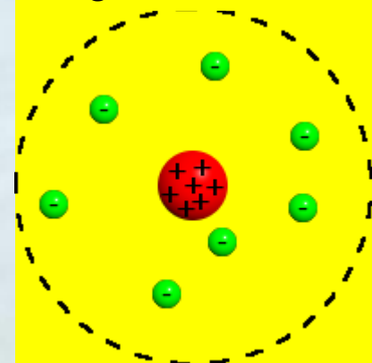
Nagaoka's atom
