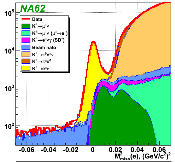
2007 data, NA48 detector
