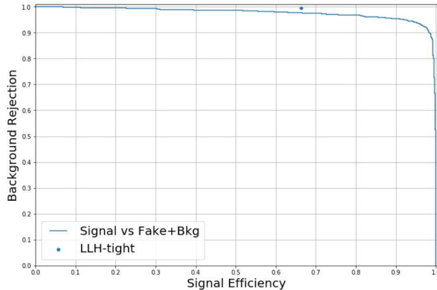
Testing Sample ROC Curve
