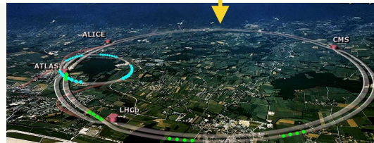
Dark matter
