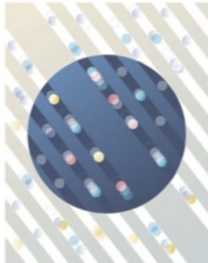
Neutrino mass
