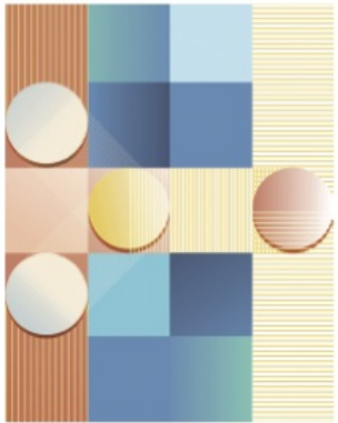
Higgs boson
