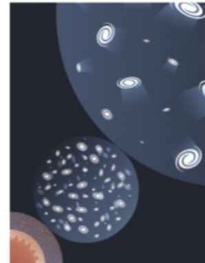
Cosmic acceleration
