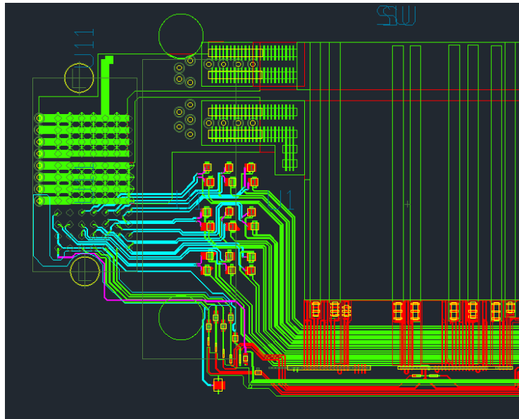
Flex interposer PCB
