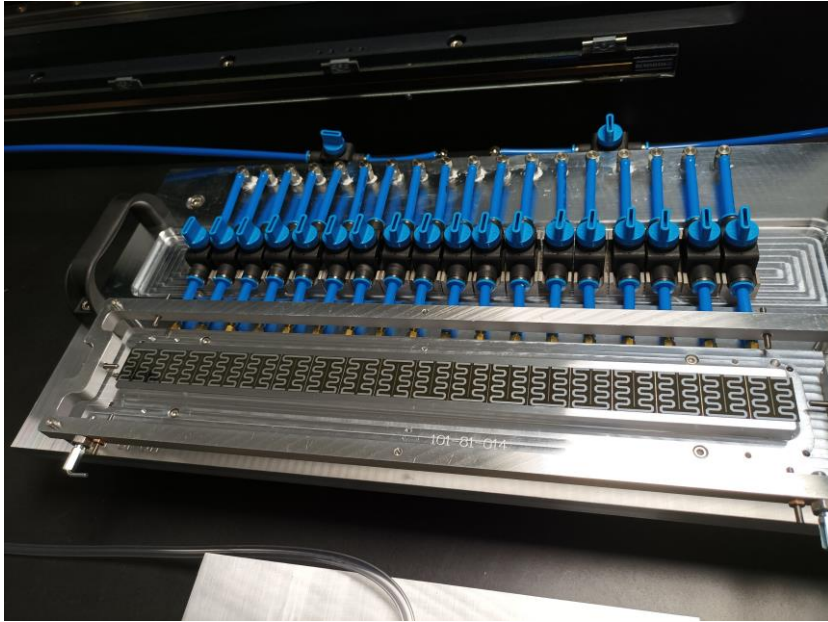
A series of 18 silicon chips aligned on the chuck. Alignment precision \sim 6 \mu\text{m} .
