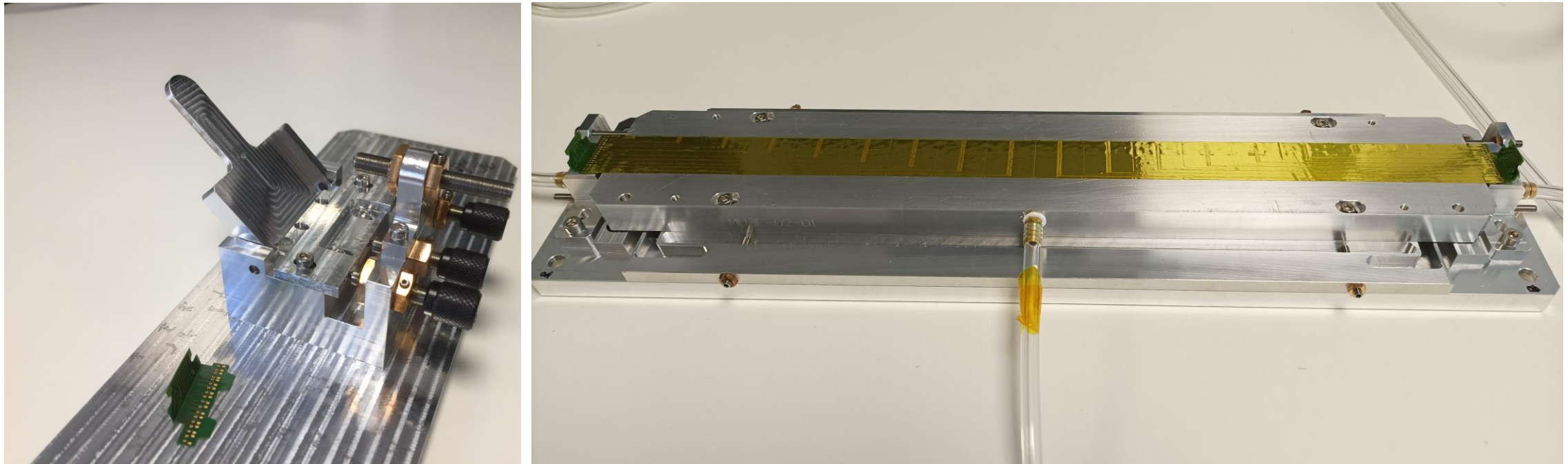
Left: flex interposer bending tooling. Right: the HDI flex is placed on a vacuum chuck and aligned against the flex interposers mounted at the ends.
