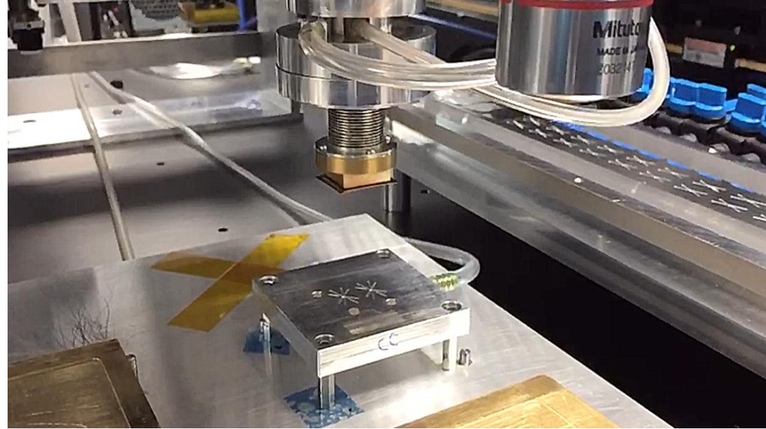
Gantry robot. Foreground: the chip base plate and the pick-up tool with camera; in the background the chip chuck.
