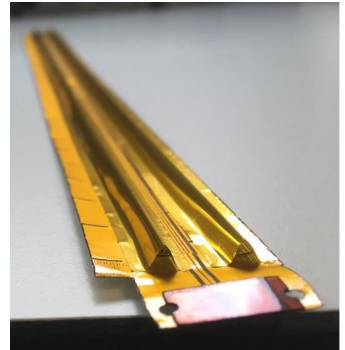
Flex tape mock-up with V-fold (right).
