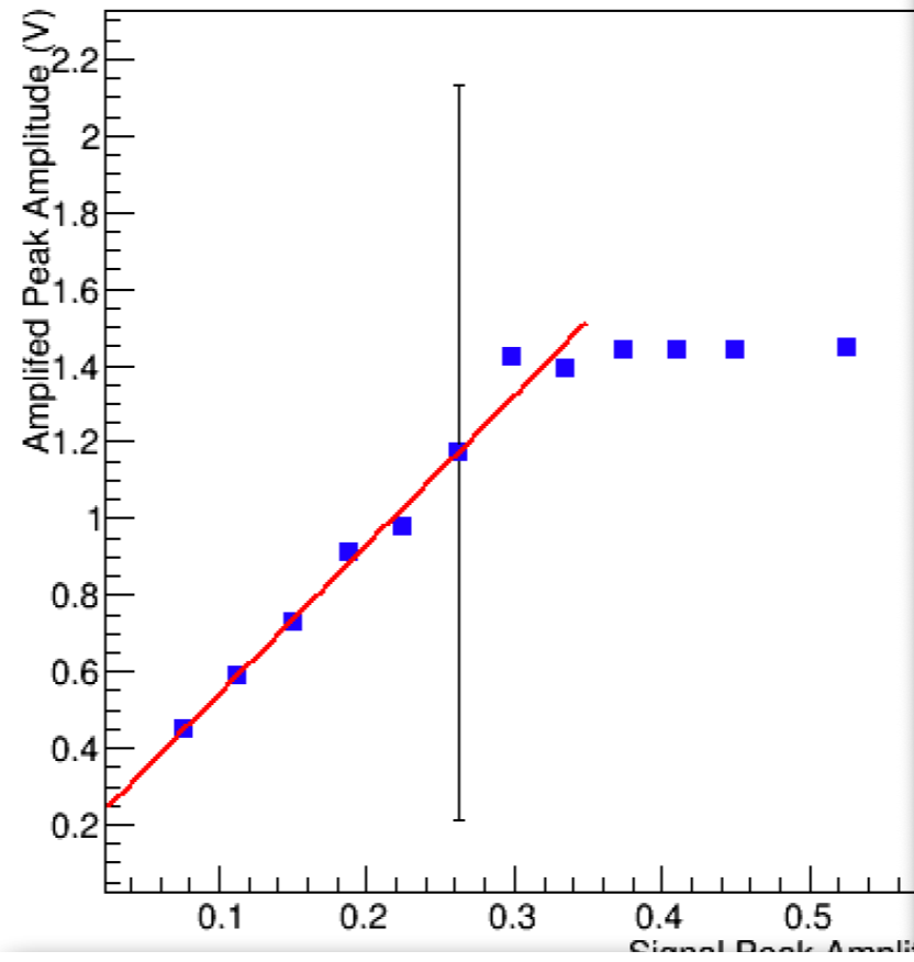
Expected Signal Rerse Recorded Peak Amplitude. Channel
