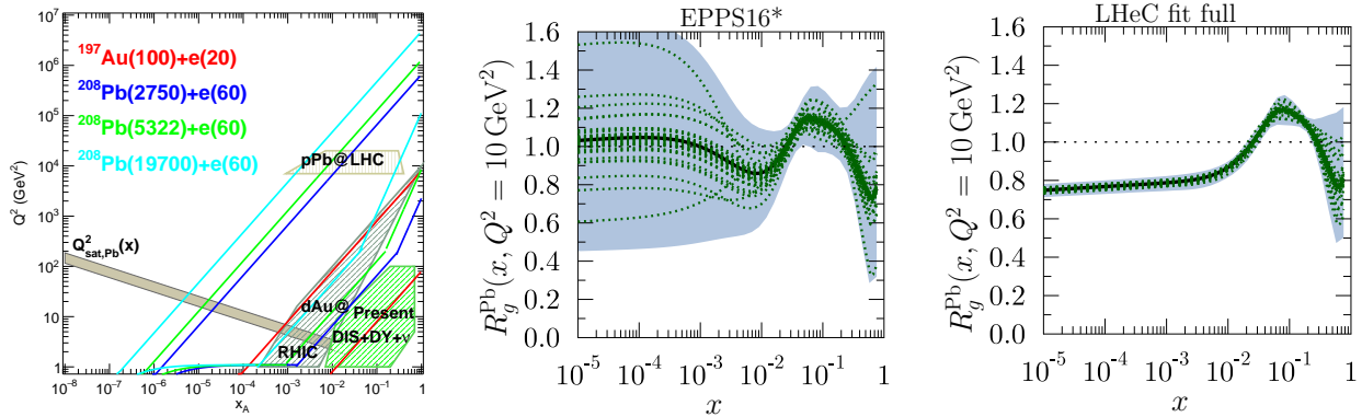
Figure 5: Left: x-Q^2 plane for future eA colliders also indicating the region covered by data used in present global fits and the estimated line of the saturation scale for Pb. Middle and right plots: Pb/p ratio of the gluon PDF in the modified EPPS16 analysis in [43], both for the present situation (middle) and including NC, CC and charm LHeC pseudo-data (right).
