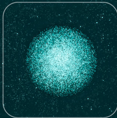
Higgs boson
