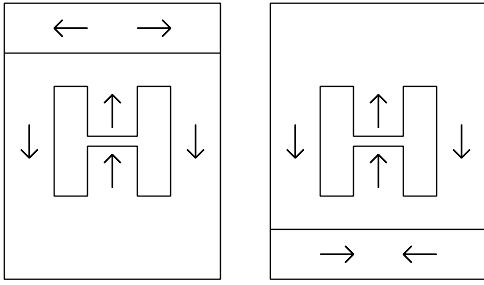
Figure 1: Alternating dipole laminations of grain oriented silicon steel. The arrows show the \mathbf{B} field direction and the grain direction. The layout resembles an “EF” transformer.
