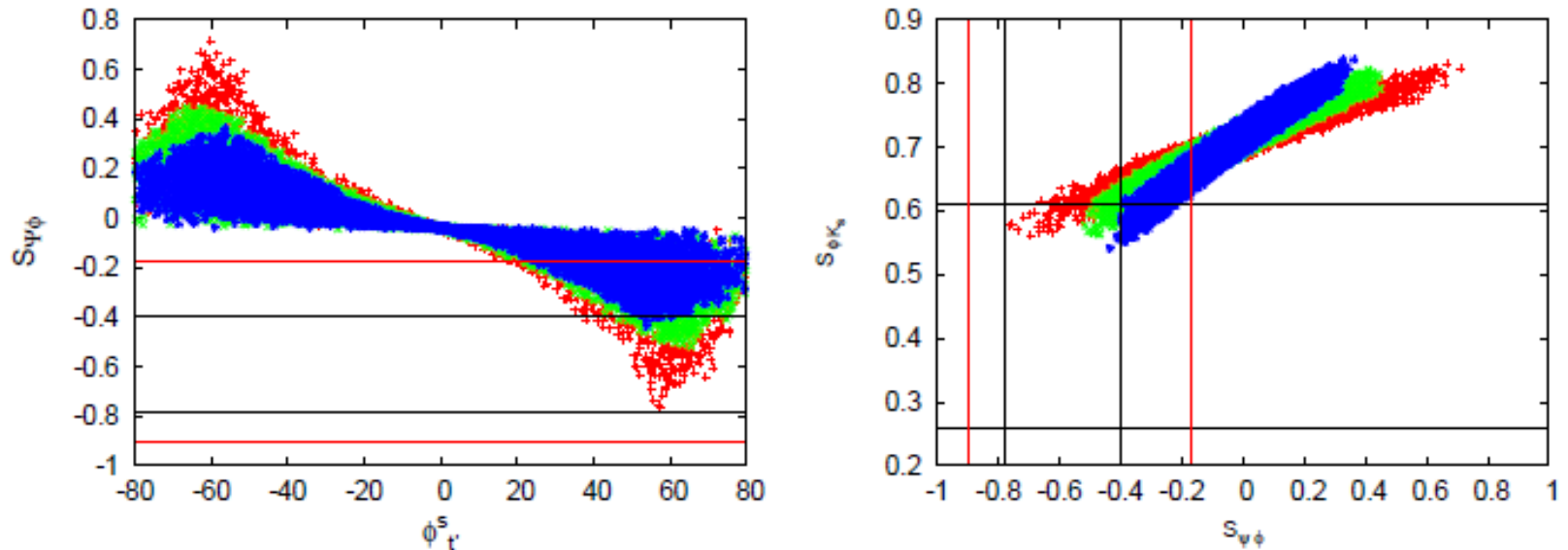
FIG. 1: The left panel shows the allowed range for S_{\psi\phi} in the (S_{\psi\phi} - \phi_{t'}^s) plane for m_{t'} = 400 (red), 500 (green) and 600 (blue) GeV respectively. Black and red horizontal lines in the figure indicate 1\text{-}\sigma and 2\text{-}\sigma experimental ranges for S_{\psi\phi} respectively. The right panel shows the correlation between S_{\phi K_s} and S_{\psi\phi} for m_{t'} = 400 (red), 500 (green) and 600 (blue) GeV respectively. The horizontal lines represent the experimental 1\sigma range for S_{\phi K_s} whereas the vertical lines (Black 1\text{-}\sigma and red 2\text{-}\sigma ) represent that for S_{\psi\phi} .
