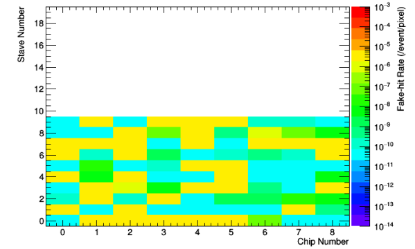
Layer-2, Run 102935 (1/157)
