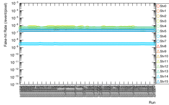
Layer-1, from_run102929_to_run103477
