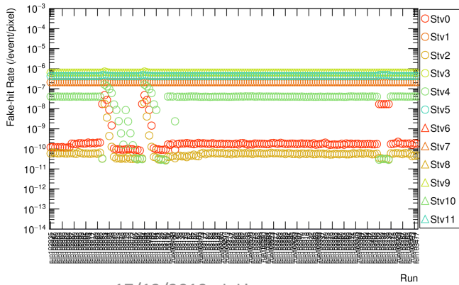
Layer-0, from_run102929_to_run103477
