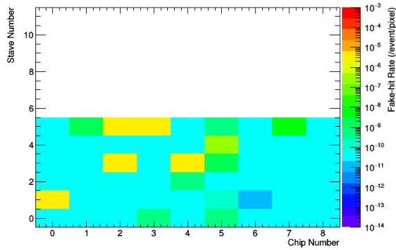
Layer-0, Run 102935 (1/157)
