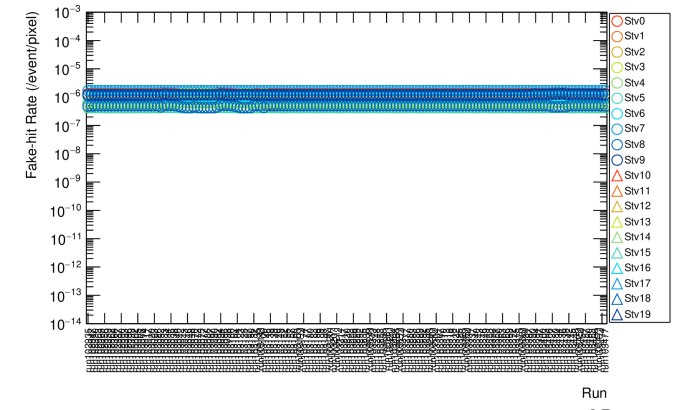
Layer-2, from_run102929_to_run103477
