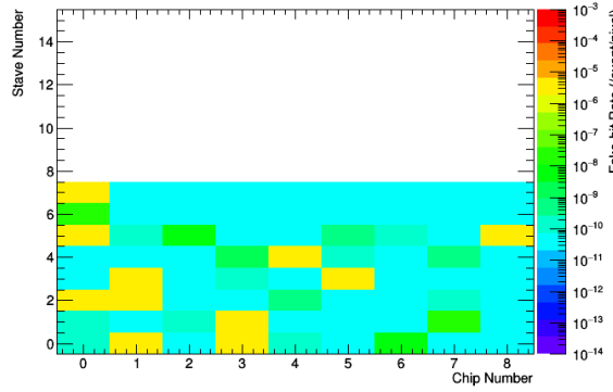
Layer-1, Run 102935 (1/157)
