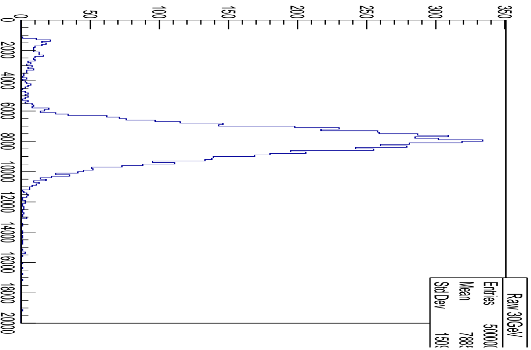
Raw 30GeV
