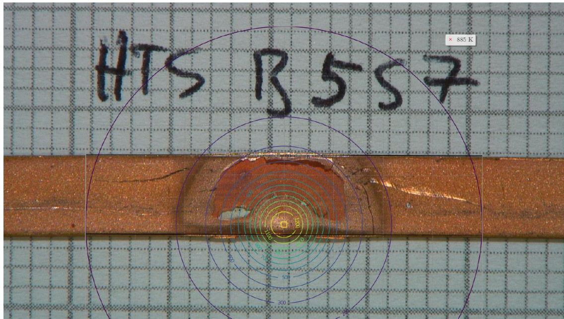
Temperature deposition curve from the FLUKA simulations overlaid the HTS B5S7 tape Credit: A. Will, A. Oslandsbotn
