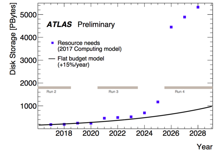
This shows Projected Disk Usage. Projected CPU usage looks very similar.
