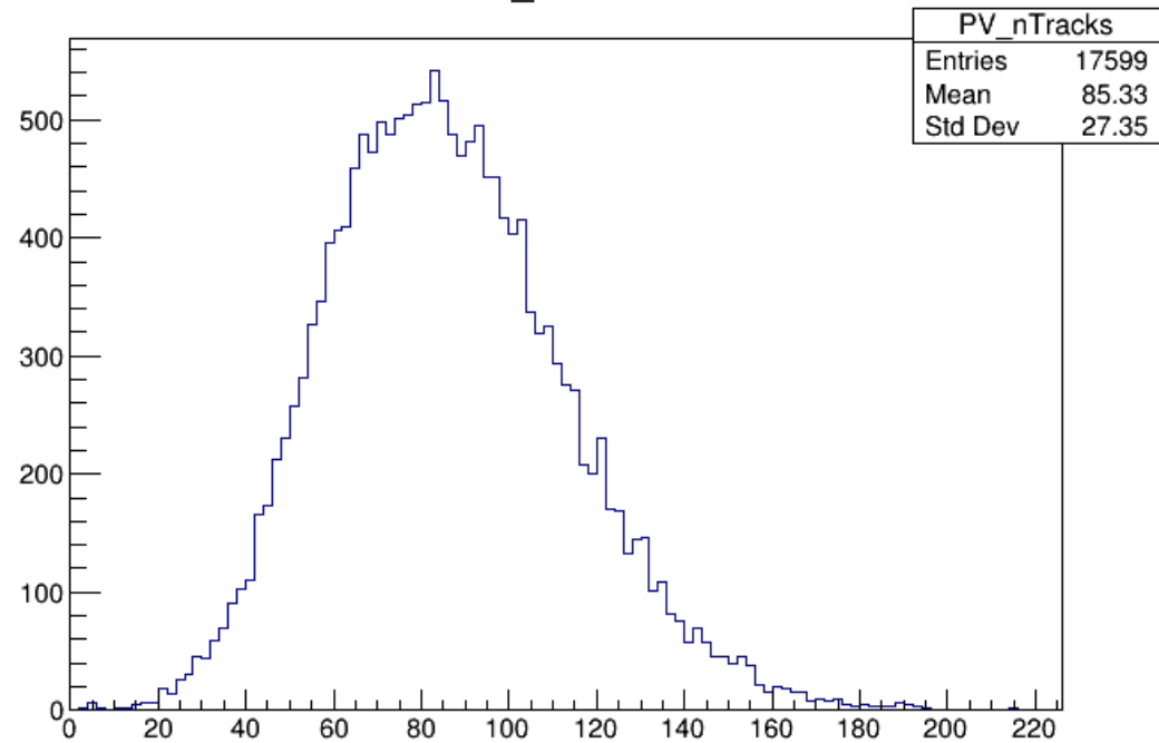
PV_nTracks
