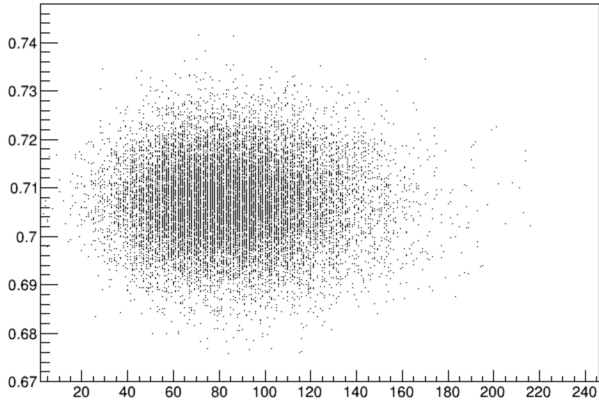
PV_r:PV_nTracks
