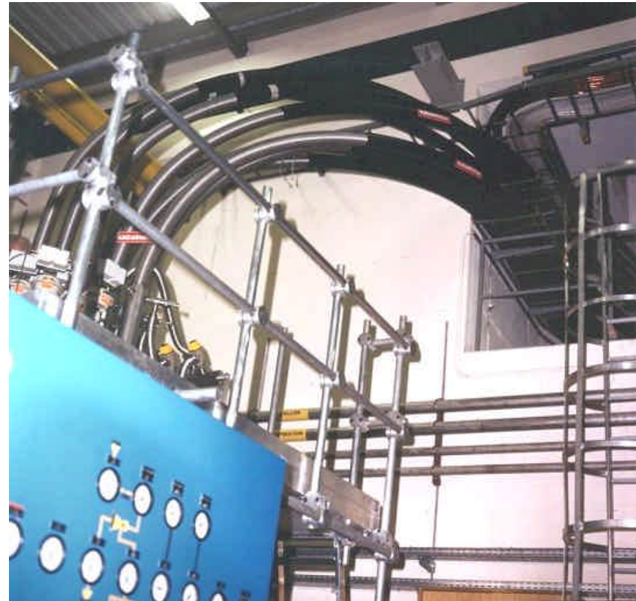
CERN 7 x 50 m LHe Transfer Lines
