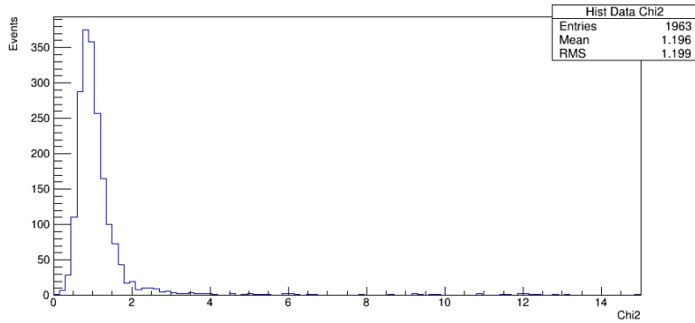
Chi-squared/dof
