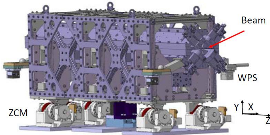
Type 4 MBQ and stabilization system mounted on cam movers (left) and test setup including ZCMs, follower girder and local coordinate system (right).
