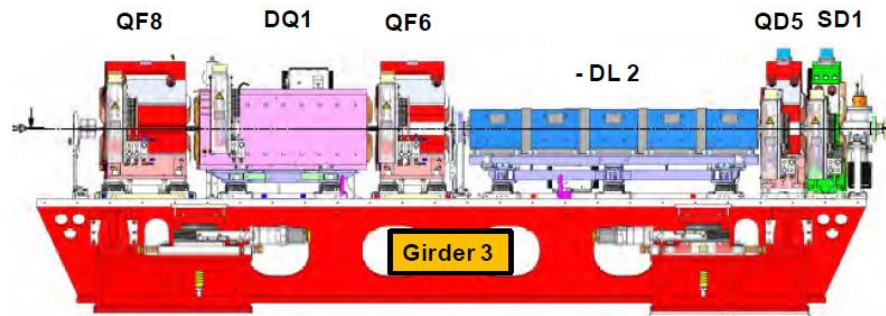
Girder 3 layout
