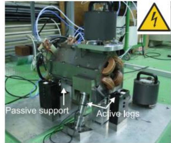
A Type 1 quadrupole magnet for CLIC on two active inclined piezo-electric actuators
