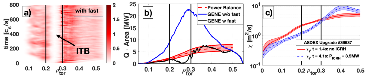
Figure 1: a) Time evolution of total ion heat flux (thermal + fast) in gyroBohm units; b) thermal ions + electrons + fast ions heat flux in MW averaged over t[c_s/a] = [400–600] ; c) radial profile of the ion conductivities computed by ASTRA.
