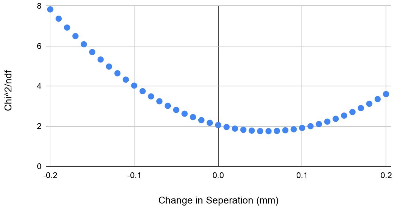
Chi 2 /ndf vs. Change in Separation (mm) (Fixed)
