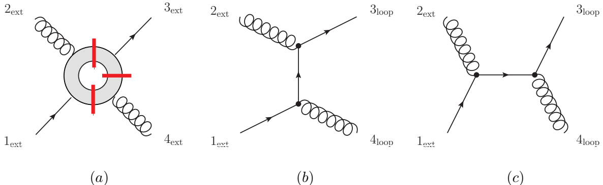
Figure 1. A triple cut of the primitive amplitude A^{\text{prim}}(\overline{Q}_1; g_2; Q_3; g_4) as shown in (a) with two three-point tree amplitudes and one four-point tree amplitude A^{\text{tree}}(\overline{Q}_{1\text{ext}}; g_{2\text{ext}}; Q_{3\text{loop}}; g_{4\text{loop}}) . The latter consists of the above two ordered tree diagrams (b) and (c). “ext” resp. “loop” denote external legs, resp. on-shell loop legs. Note the absence of any gluon self interactions.
