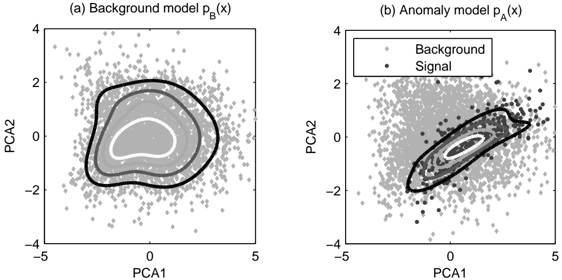
Figure 3. (a) A projection of the WH background data into its two-dimensional principal subspace. The solid lines show contours of the estimated 5-component Gaussian mixture model for the background. (b) A projection of the m_H = 150 GeV test data set into the two-dimensional principal subspace. The solid lines show contours of the estimated 2-component Gaussian mixture model for the signal.
