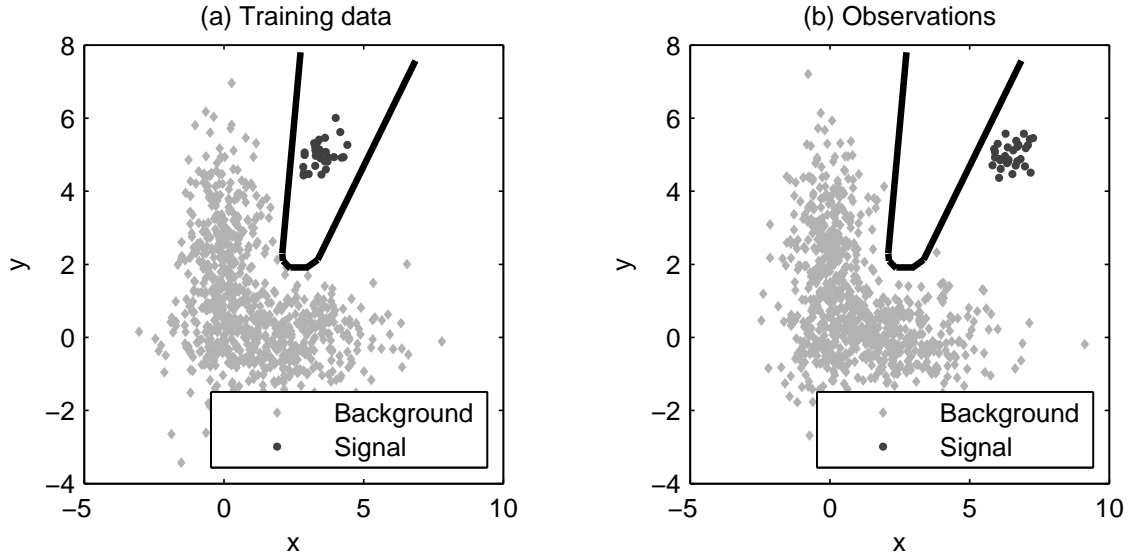
Figure 1. Demonstration of the limitations of model-dependent searches of new physics. When a neural network is trained with the data of figure (a), the classification decision boundary is given by the black curve. But if the training data is systematically inaccurate, the new physics signal could be completely missed in the analysis. For example, all the observations of figure (b) would be classified as background.
