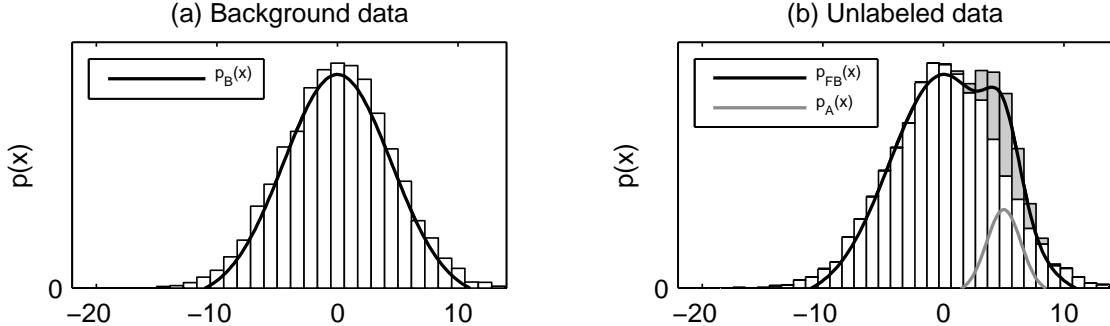
Figure 2. (a) A histogram of background data from a univariate Gaussian distribution and an estimated background model p_B(x) . (b) An illustration of the fixed-background model in a univariate case. The histogram shows the unlabeled observations (the gray excess in the histogram denotes the anomalous contribution). The estimated fixed-background model p_{FB}(x) is shown with a black line and the anomaly model p_A(x) with a gray line.
