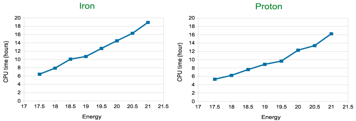
Figure 3. Left: CORSIKA average execution time as a function of the logarithm of the energy for iron primary cosmic rays. Right: same plot for proton cosmic rays
