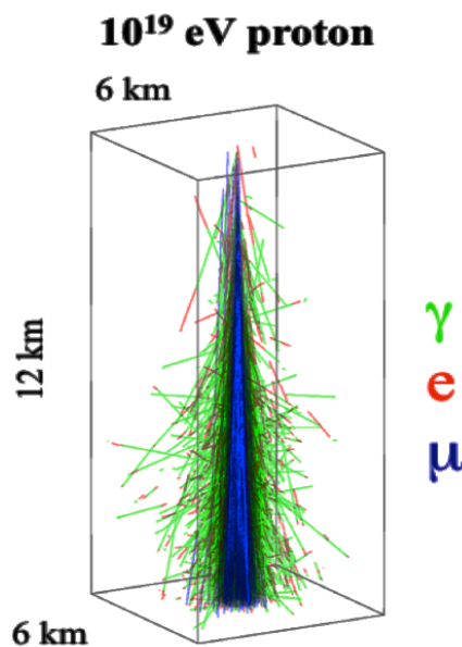
Figure 2. Image showing the development of a single EAS produced by a proton with an energy of 10^{19} eV. Most prominent particle types are shown in different colours [2]
