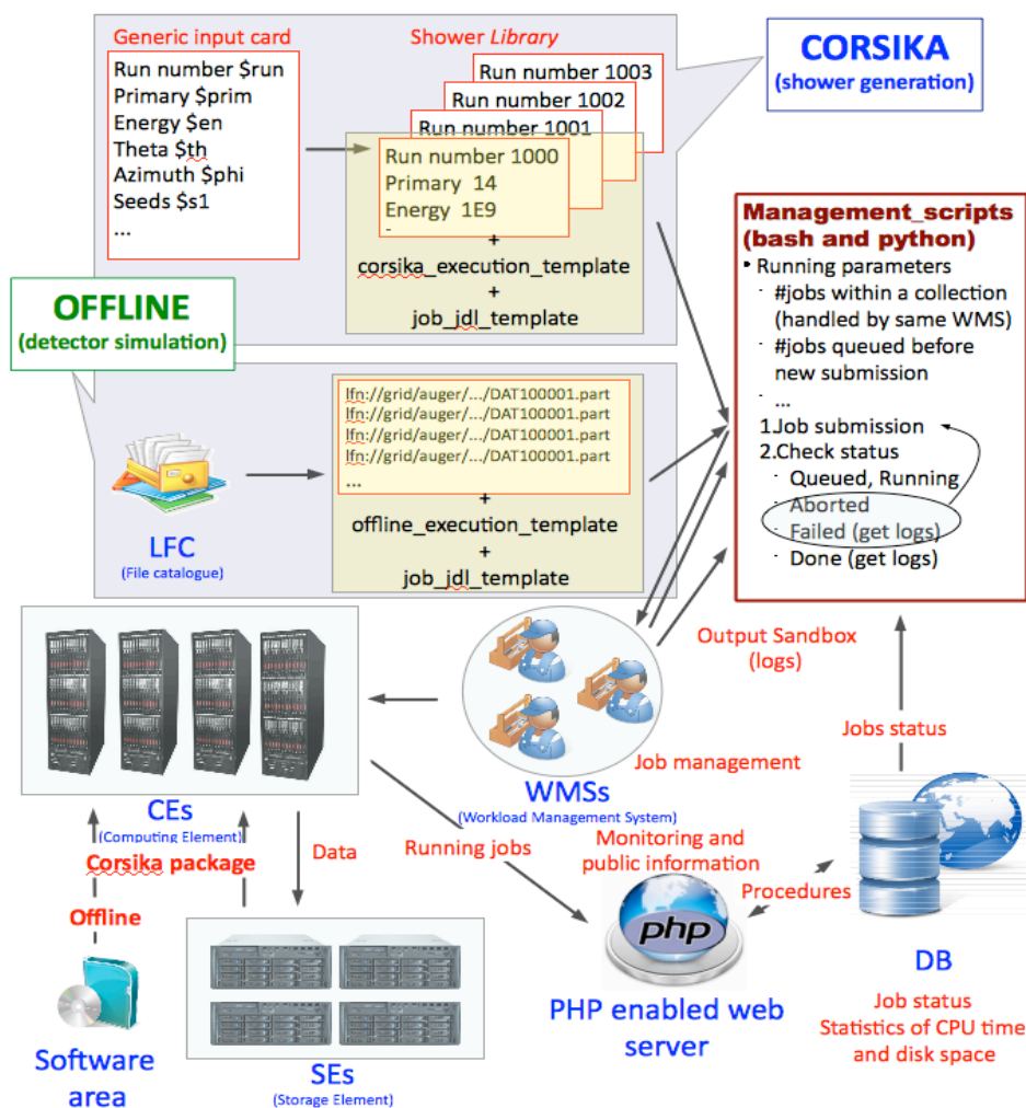
Figure 7. Workflow of the Auger simulation productions
