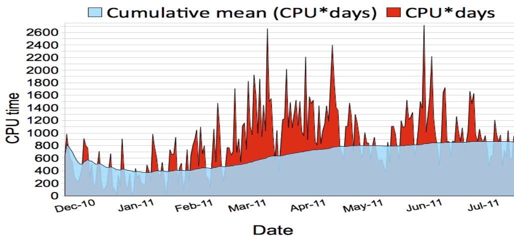
Figure 8. Daily CPU and cumulative mean CPU consumption of the Auger VO since end of 2010
