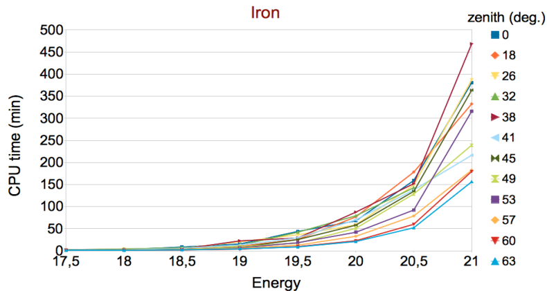
Figure 5. CPU time of an Offline execution as a function of the energy for various zenith angles
