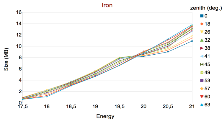
Figure 6. Total size of Offline output files as a function of the energy for various zenith angles
