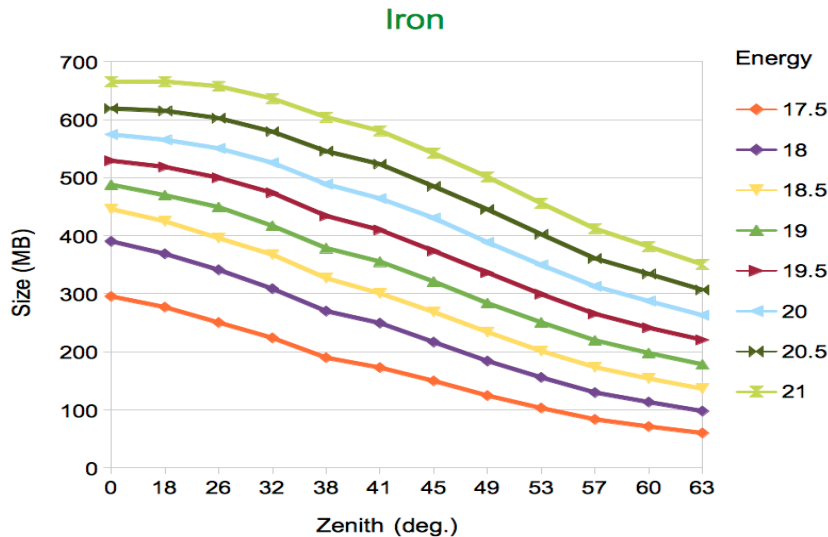
Figure 4. Size in MBs of the output files containing information on generated showers as a function of the zenith angle of the primary for iron primaries at diverse energies (expressed as \log(E) )
