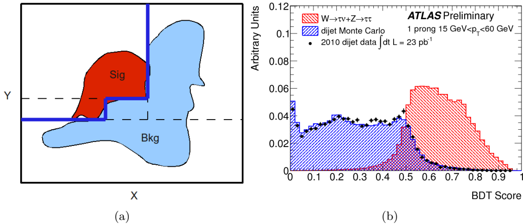
Figure 5: (a) Illustration of a piecewise continuous cut through a 2D plane made by a simple decision tree. Signal is in red, background in blue. (b) BDT discriminant output scores for signal and background for 1-prong \tau candidates [2].
