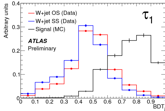
Figure 8: Templates used to extract signal cross section in t\bar{t} analysis [8].
