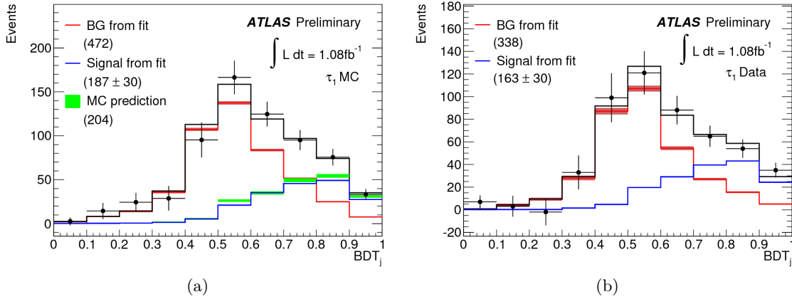
Figure 9: Results of template fits from the t\bar{t} \rightarrow \mu + \tau + X analysis. (a) The fits performed on simulation only, (b) The fits performed on data [8].
