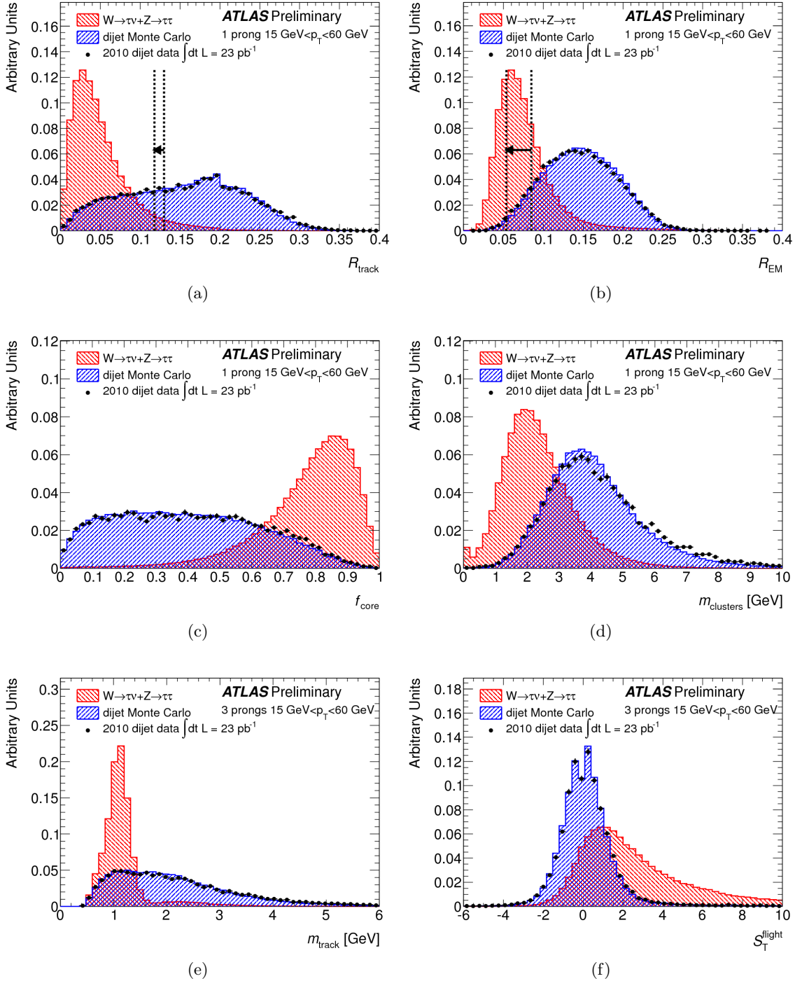
Figure 3: Variable distributions used to separate hadronic \tau from quark and gluon jets [2]. (a) Track radius (b) Electromagnetic radius (c) Core energy fraction (d) Cluster mass (e) Track mass (f) Transverse flight path significance.
