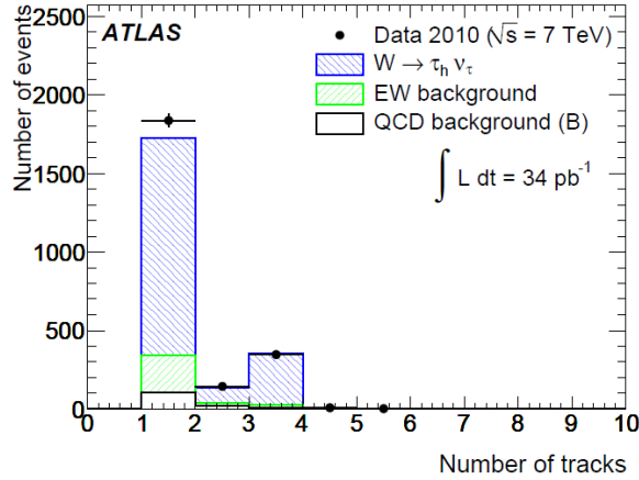
Figure 7: The number of charged tracks reconstructed as part of the \tau candidate. True \tau should have an odd number of associated tracks (charge conservation) [7].
