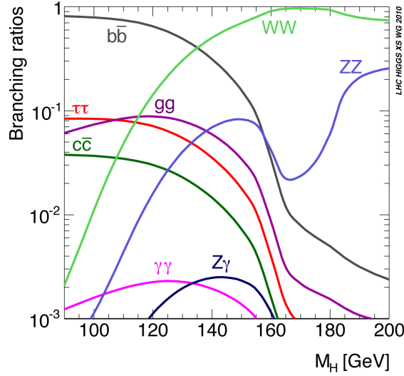
Figure 1: Standard Model Higgs branching ratios as a function of the mass of the Higgs [1].
