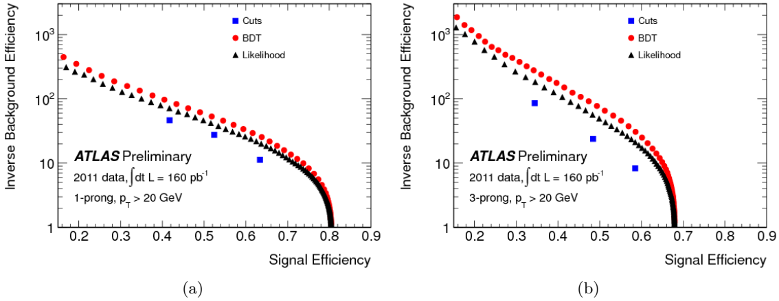
Figure 6: Performance summary for three different techniques to separate \tau from jet backgrounds: cuts, LLH and BDT. (a) 1-prong candidates (b) 3-prong candidates. Taken from [6].
