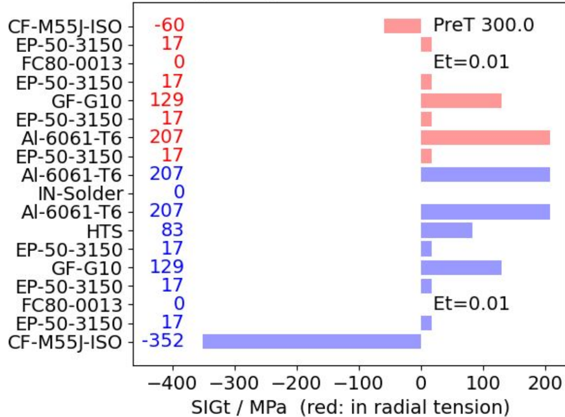
LargeCoil_24 4K Azimuthal Stress
