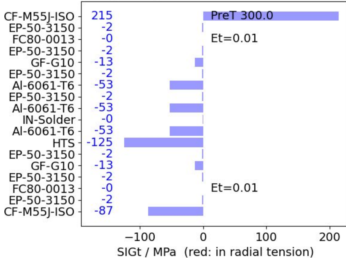
LargeCoil_24 293K Azimuthal Stress
