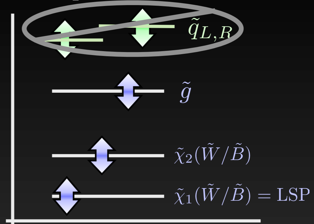
Mass spectrum
