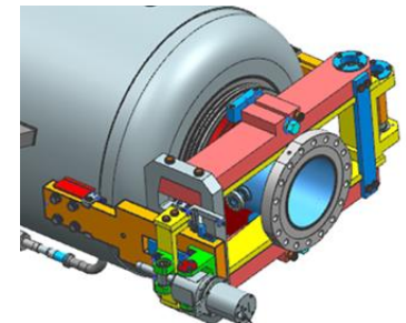
650 MHz cavity tuner
