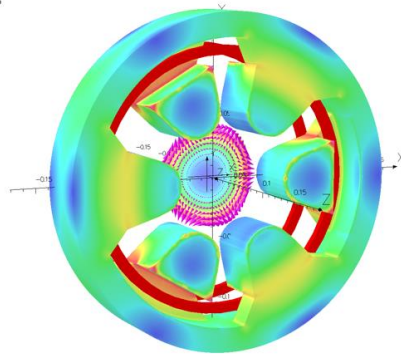
Double Coil Sextupole
