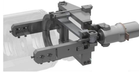
1.3 GHz cavity tuner
