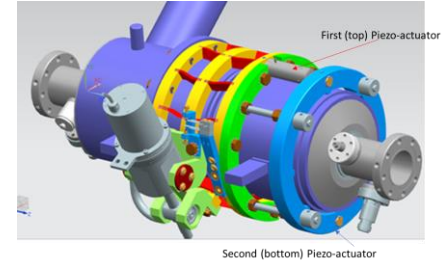
3.9 GHz cavity tuner
