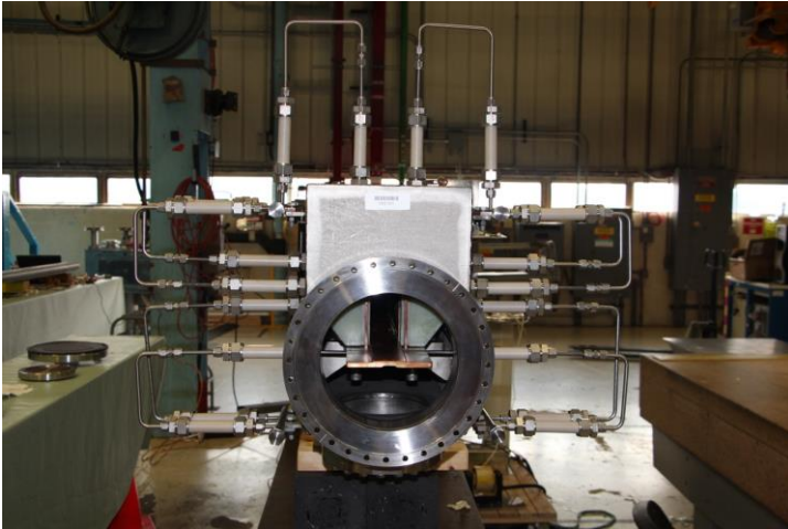
Pulsed septum magnet for muon delivery ring
