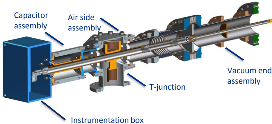
SSR2 FPC assembly
