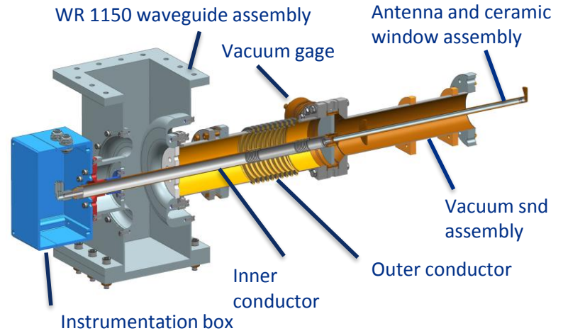
HB650 FPC assembly
