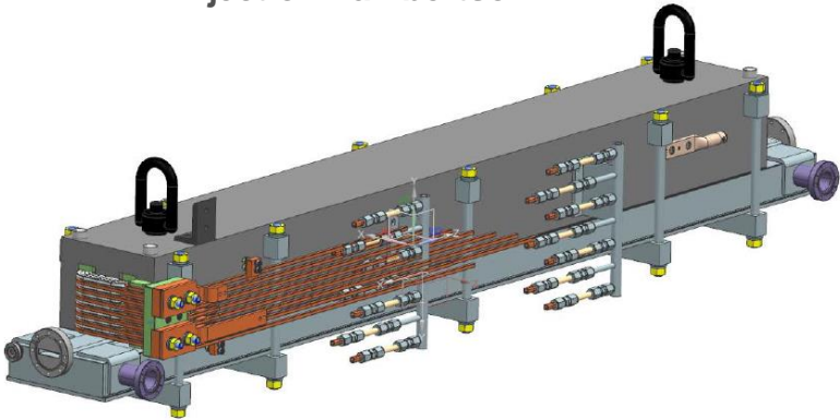
Injection Lambertson
