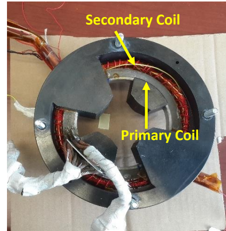
HTS quadrupole test setup
