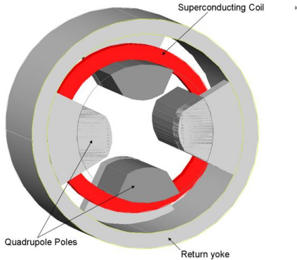
Single coil quadrupole
