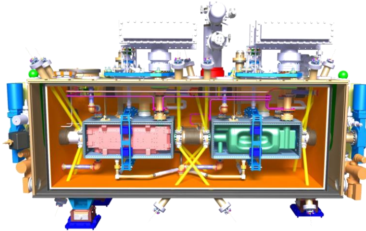
Cryomodule Design (CERN)
