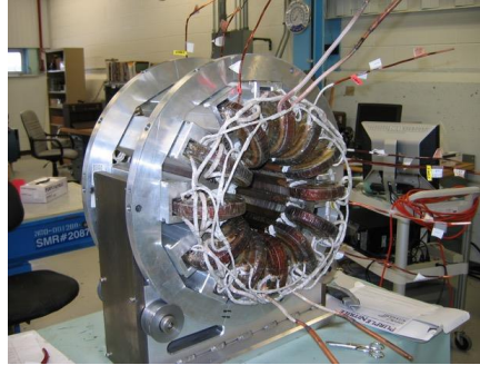
Six magnets in one package
