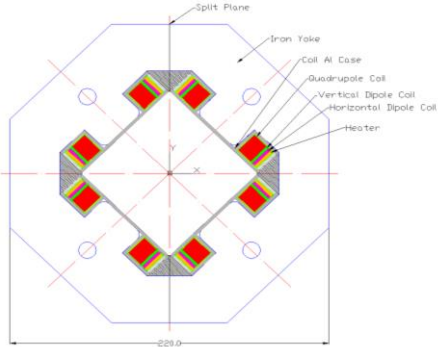
Magnet cross-section
