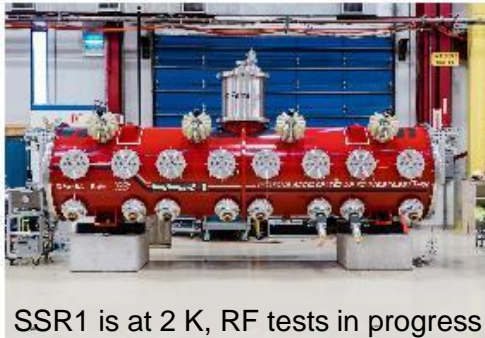
Single Spoke Resonator (SSR1)
