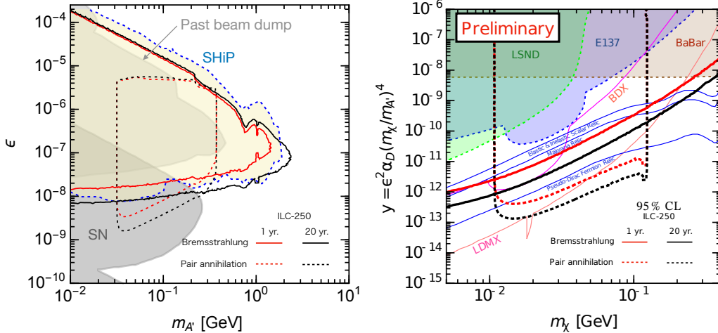
Figure 5: Expected sensitivity of main beam dump experiments at the 250 GeV ILC after one year (red lines) and 20 years (black lines) of running to processes with dark photon production with visible dark photon decays (left) [11] and invisible decays to DM particles (right) [13].
