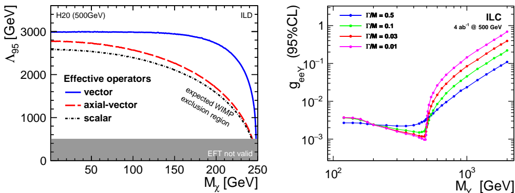
Figure 2: The expected sensitivity of the ILD experiment, for ILC running at 500 GeV, to DM pair production. Left: EFT limits on mediator mass scale \Lambda as a function of the DM particle mass M_\chi , for different mediator types [7]. Right: mediator coupling limits as a function of the vector mediator mass M_Y for DM particle mass M_\chi=50 GeV [8].
