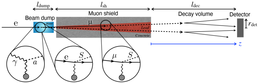
Figure 3: An experimental setup proposed for new light particle searches at the ILC [10].
