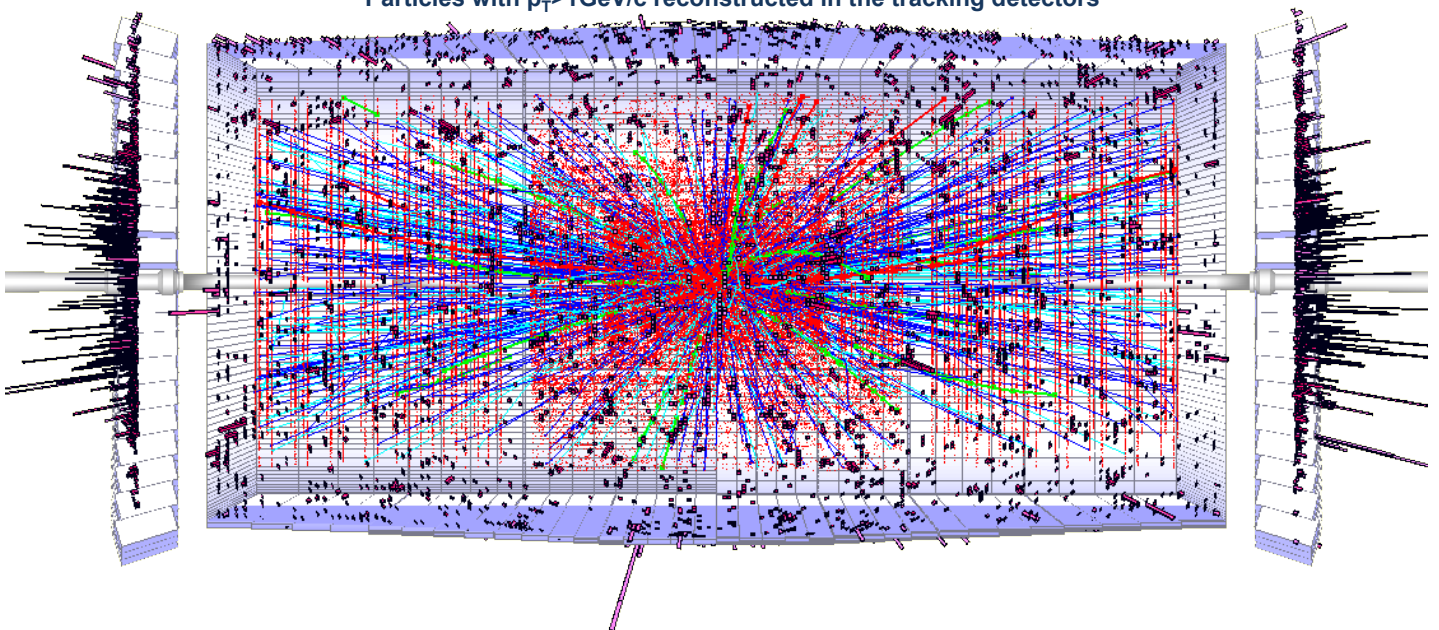
High-Luminosity bunch crossing with 200 pp collisions Particles with p_T > 1\text{GeV}/c reconstructed in the tracking detectors
