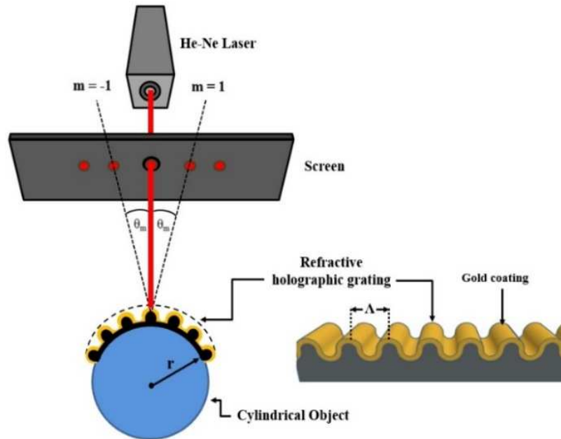
14 Figure 1. The schematic diagram for measuring the radius of the cylindrical object.
