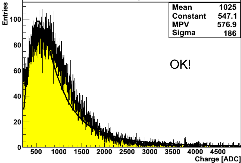
HMPID MIP Charge distribution
