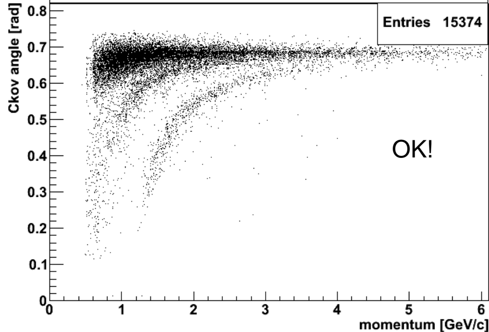
HMPID: ThetaCherenkov vs P
