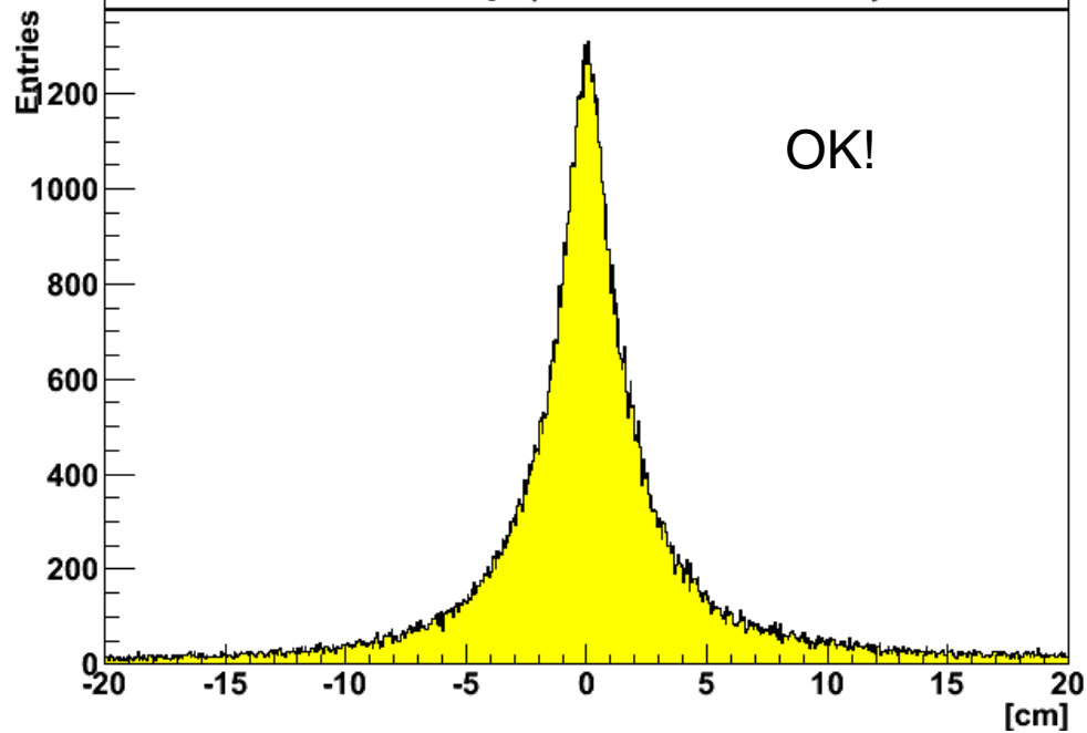
Xtrk - Xmip (local coordinate)
