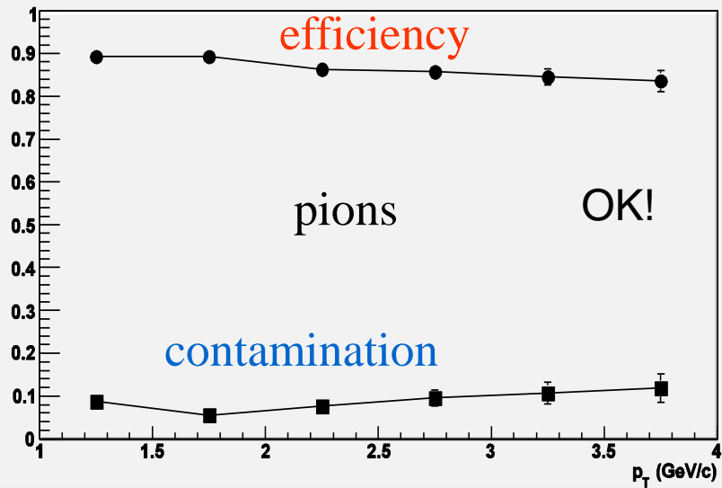
Pions
