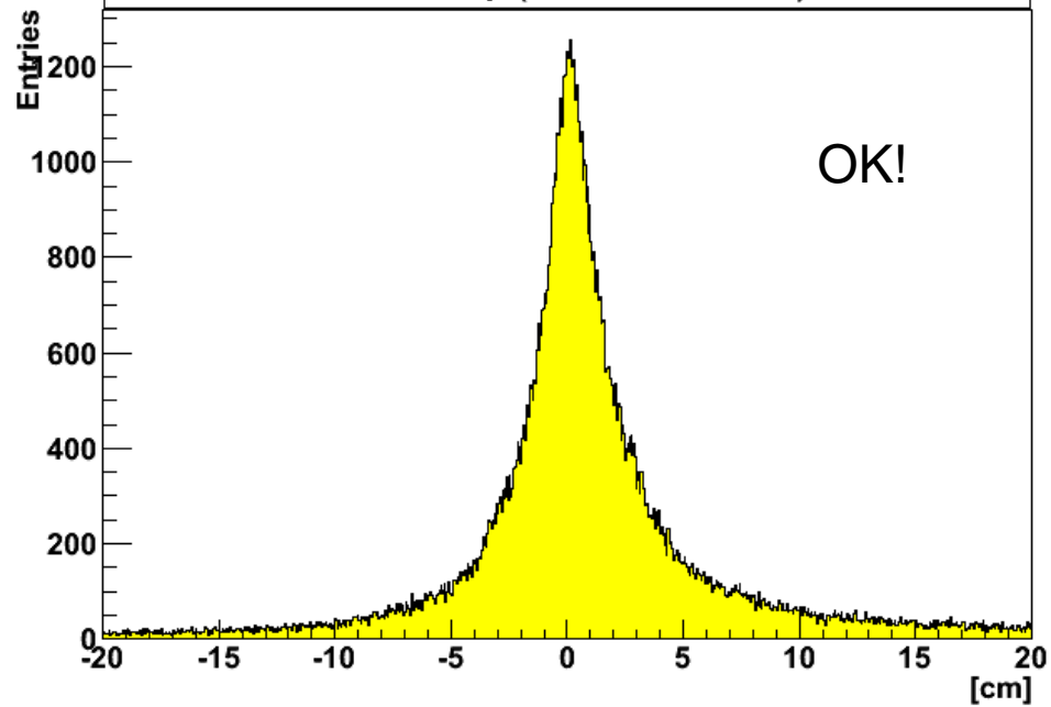
Ytrk - Ymip (local coordinate)
