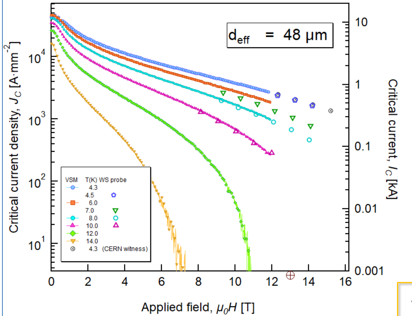
Fig. 7. The in-field behaviour of the critical current in the temperature range 4.3-14 K. Transport data have been rescaled with the ESE scaling law.
