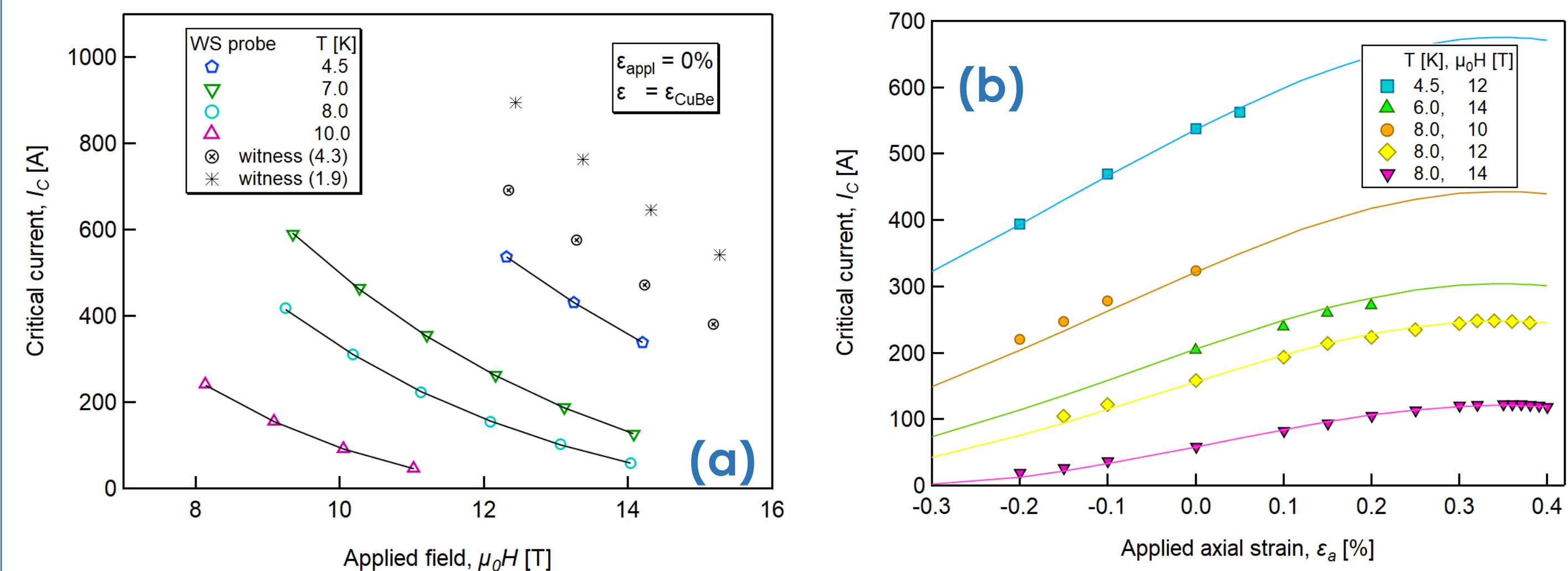
Fig. 4. I_c vs.: (a) peak field, at different temperatures and \epsilon_{\text{appel}}=0\% ; (b) applied strain, at different temperature and external magnetic fields. The continuous lines represent fits to the ESE parameterization by a Multi-Step Scaling approach.
