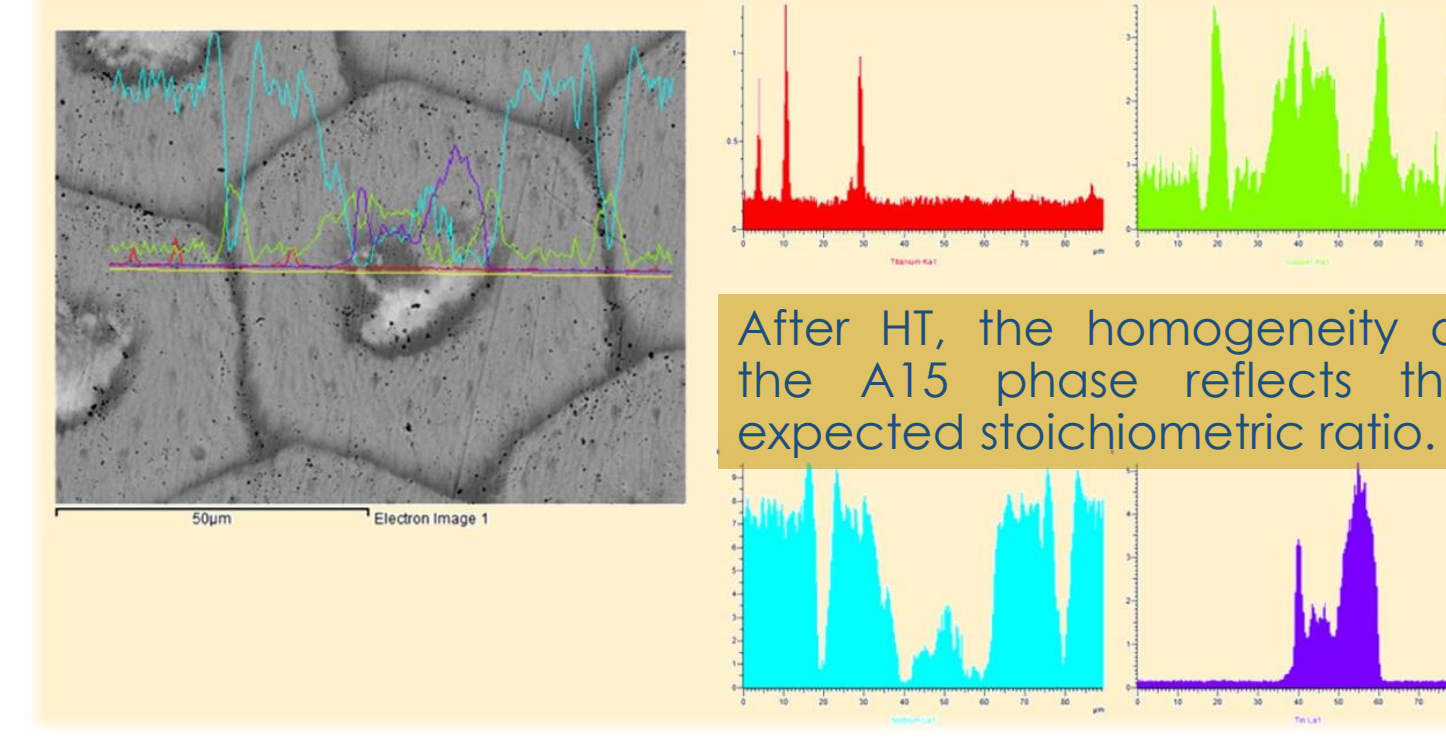
Figure 2. EDS analysis made on a selected Nb 3 Sn sub-element before heat treatment.
